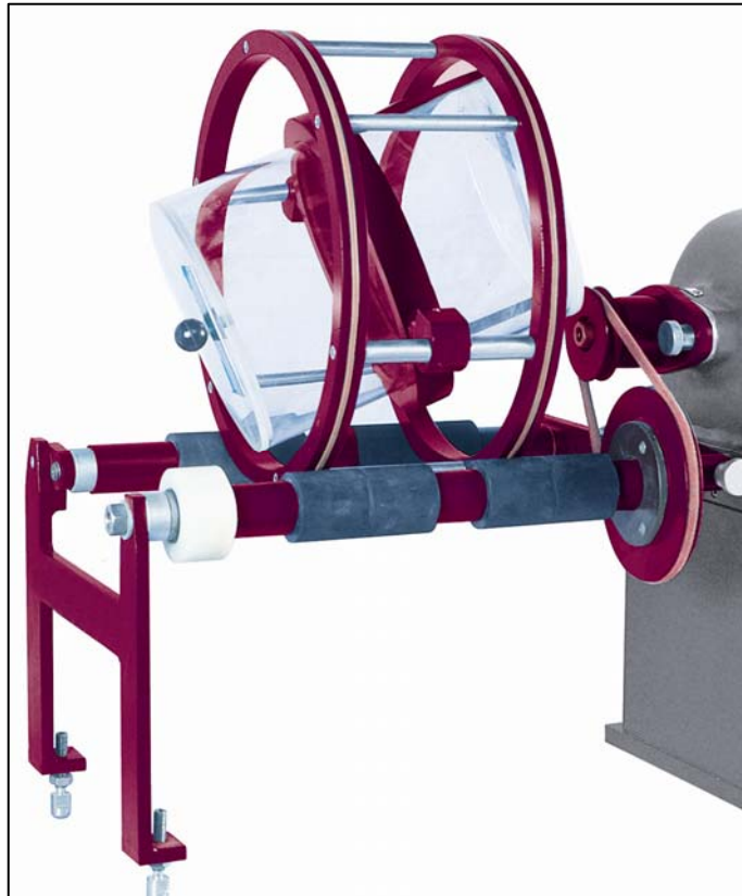
UAM Motor Drive and Drum Hoop Blender HM-5
